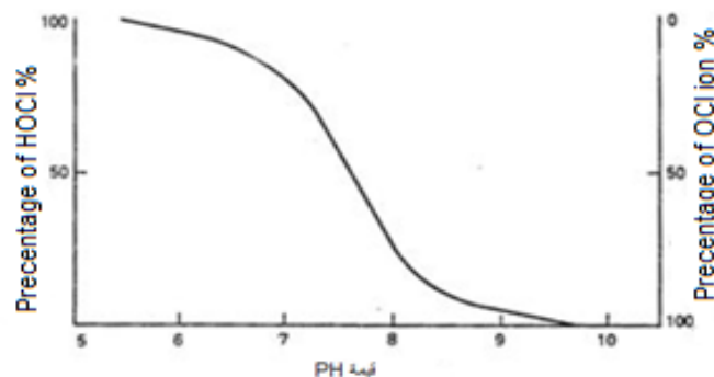
Fig.( 2):- Relationship of the ratio of HOCl to OCl^- in water at different values of PH
