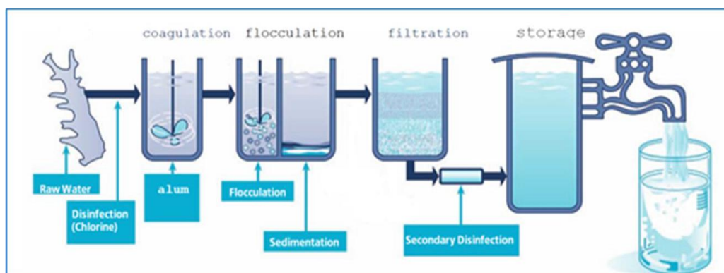
Fig(1):- Sequence of basins in drinking water purification plants
