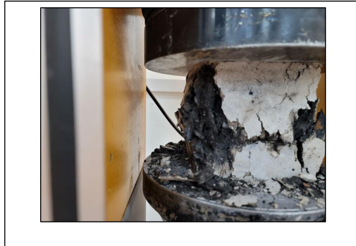
Fig.(7):- Chemical composition change of mix HSGC-4 after exposure to 1000 °C
