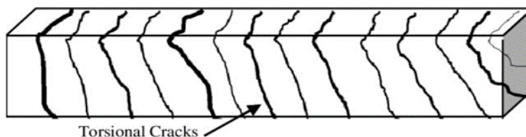
Fig.( 14):- Torsional crack
