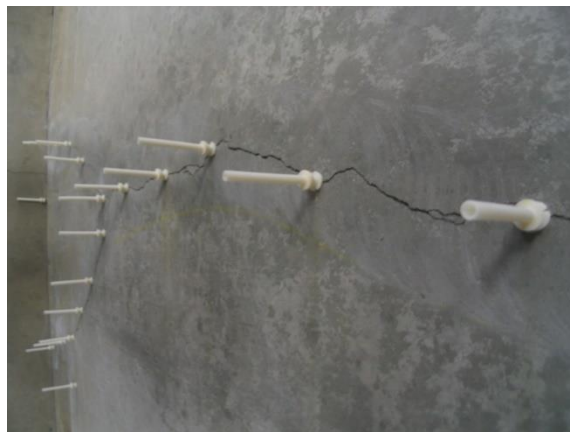
Fig.( 1):- Epoxy injection [45].
