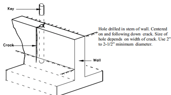
Fig.( 15):- Drilling and plugging technique [44].
