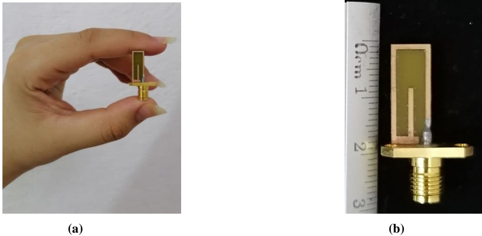
Fig.( 3) (a) .fabricated antenna for the hand (b) . The manufactured antenna relative to a ruler
